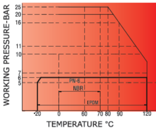
PRESSURE/TEMPERATURE DAIGRAM
